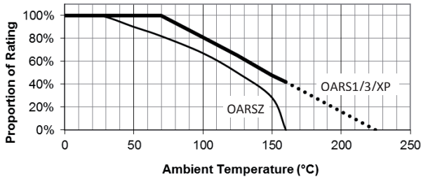
Temperature Derating
