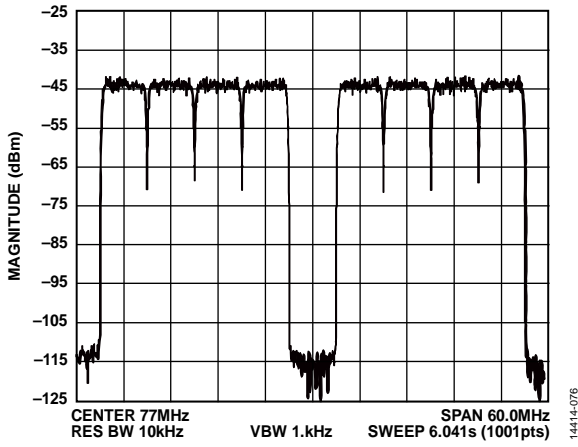
Figure 84. Gap Channel ACLR at 77 MHz
