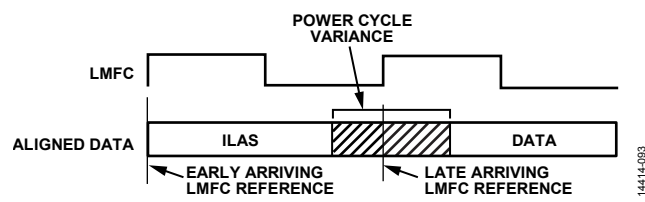
Figure 103. Link Delay > LMFC Period Example
