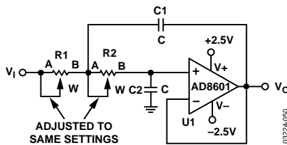
Figure 47. Sallen Key Low-Pass Filter
