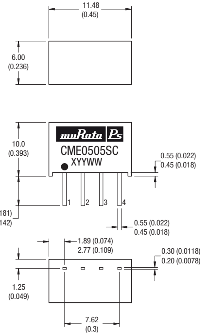
SC Package
