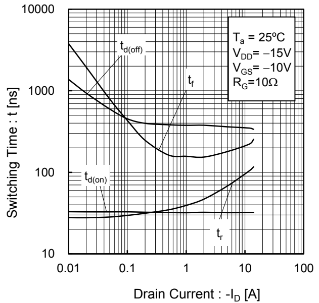
Fig.21 Switching Characteristics
