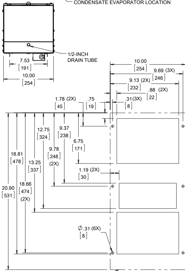
Cutout Dimensions (Externally Mounted)
