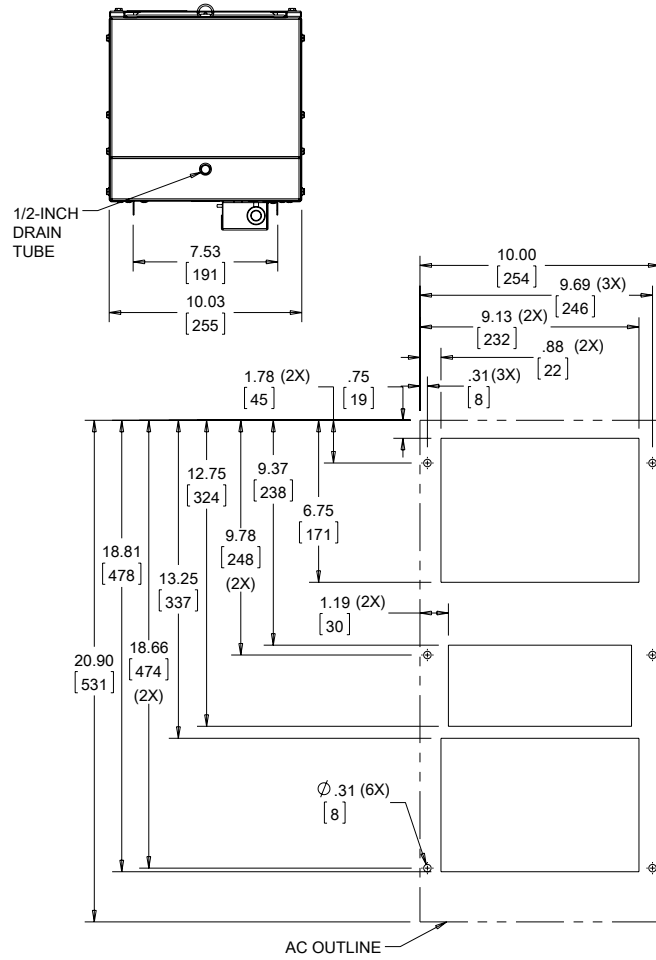
Cutout Dimensions (Externally Mounted)
