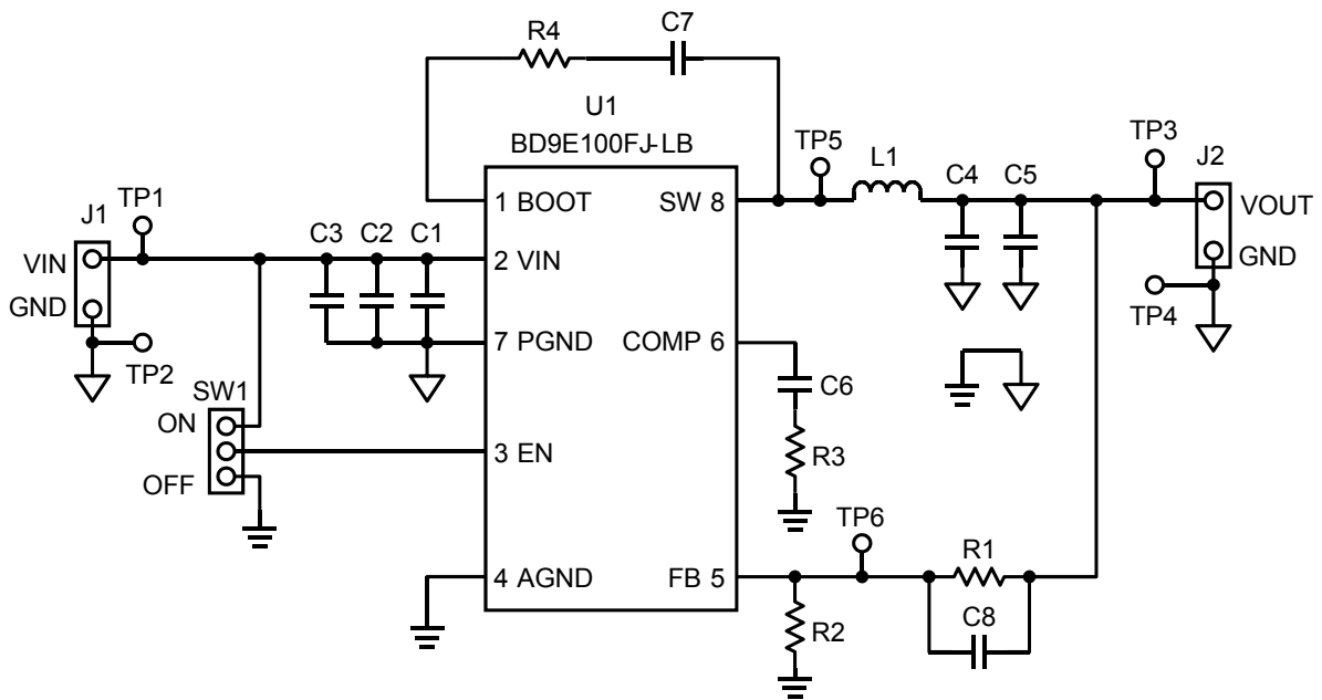
Figure 2. BD9E100FJ-EVK-001 Circuit Diagram
