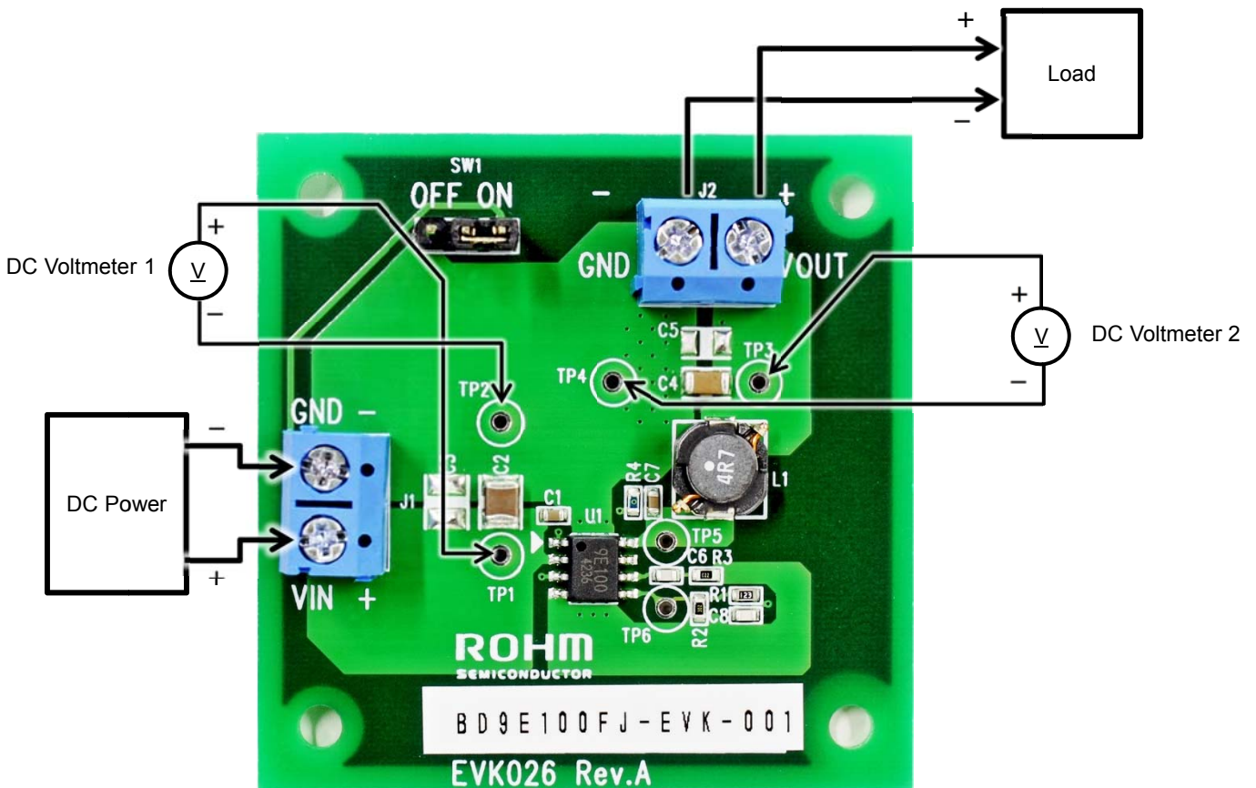
Figure 1. Connection Diagram
