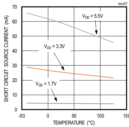
SHORT CIRCUIT SOURCE CURRENT vs. TEMPERATURE
