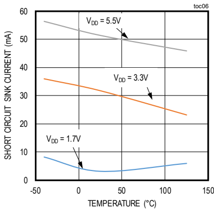
SHORT CIRCUIT SINK CURRENT vs. TEMPERATURE
