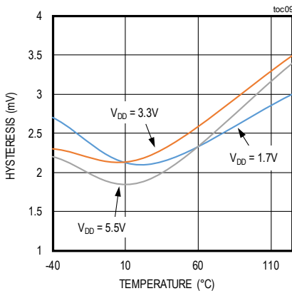
HYSTERESIS vs. TEMPERATURE
