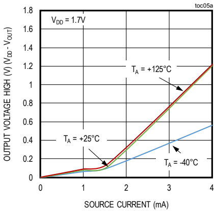
OUTPUT VOLTAGE HIGH vs. SOURCE CURRENT
