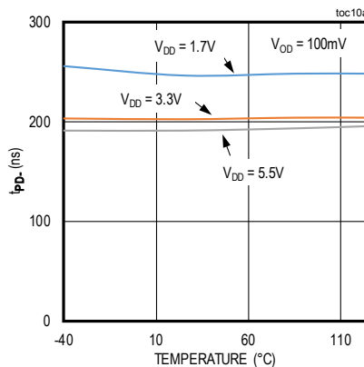
PROPAGATION DELAY (tpd-) vs. TEMPERATURE
