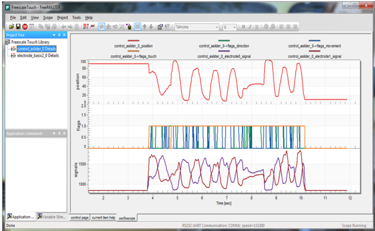
Figure 4: FreeMASTER example
