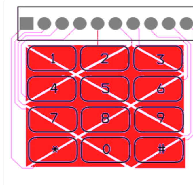
Figure 7.1.3: Keypad Electrodes
