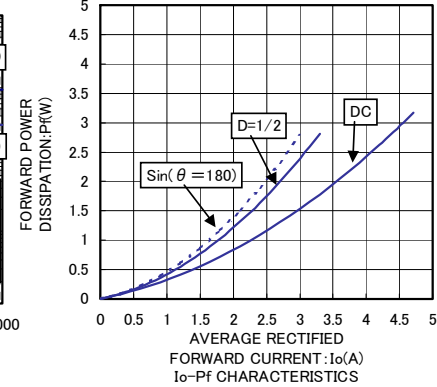
Io-Pf CHARACTERISTICS
