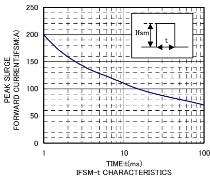
IFSM-t CHARACTERISTICS
