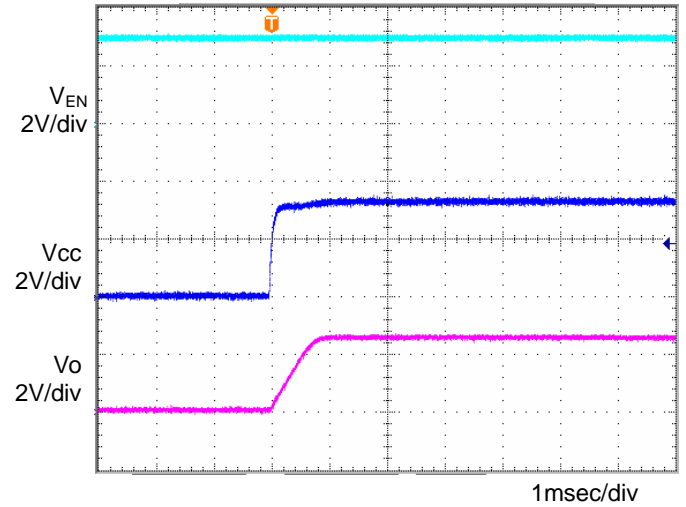
Fig.10 Input sequence 1 C_o=1\mu F, T_a=25^\circ C
