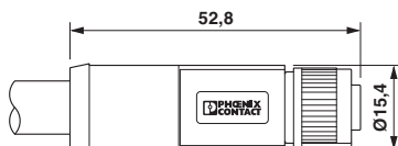
Dimensional drawing
