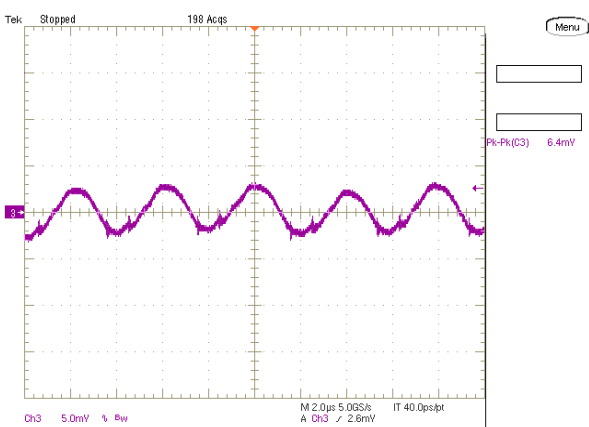
Output Ripple and Noise (Vin=5.0V, Vout=1.0V, Iout=6A, Clod=400uF, ScopeBW=20MHz)
