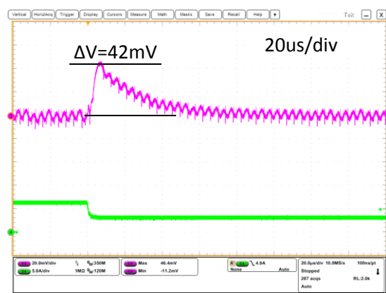
Step Load Transient Response (Vin=5.0V, Vout=0.7V, Cload=400uF, Iout=3A to 6A, 2.5A/us) Trace 3=Vout, 20 mV/div, Trace 4=Iout, 5A/div.
