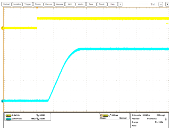
On/Off Enable Delay (Vin=5.0V, Vout=1.0V, Iout=6A, Clod=400uF) Trace1=Enable, Trace2=Vout, 2 ms/div
