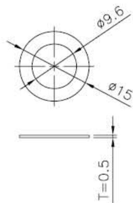
WASHER
