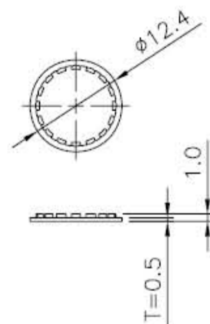
WASHER
