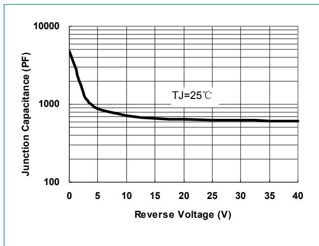
Figure 1: Typical Junction Capacitance
