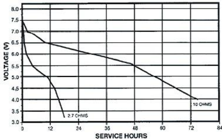
TYPICAL DISCHARGE CHARACTERISTICS 21°C (70°F)
