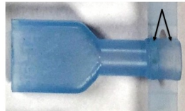
Revised 16-14 AWG standard flare part (shown here with optional carrier strip attached)
