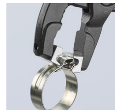
Opening a hose clamp without limit stop
