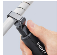
Spiral cutting
