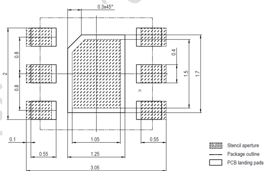
Figure 10 Recommended landing pattern.
