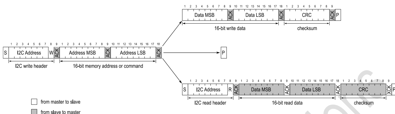
Figure 7 Communication sequence for starting a measurement and reading measurement results.
