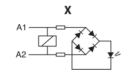
LED consumption: 1 mA
