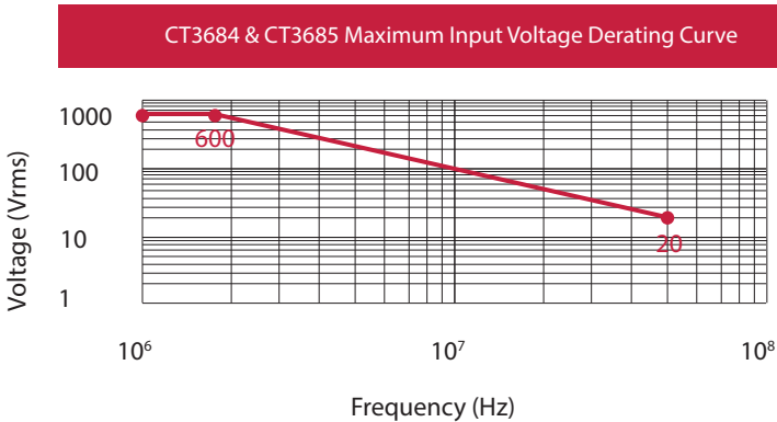
Figure 3 Derating Curve
