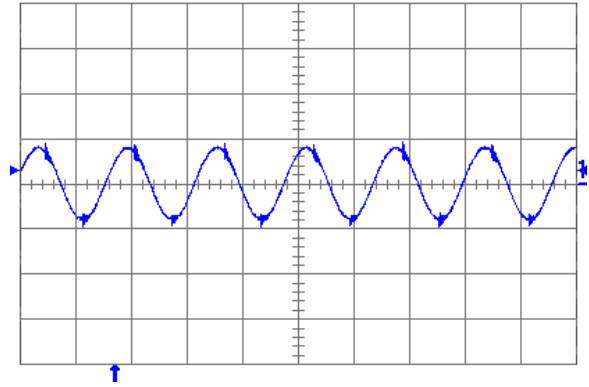
Fig. 1.8V.6: Output voltage ripple (20 mV/div.) at full rated load current into a resistive load with external capacitance 100\ \mu\text{F} ceramic + 1\ \mu\text{F} ceramic and V_{in} = 5\text{ V} for V_{out} = 1.8\text{ V} . Time scale: 2 \mu\text{s} /div.
