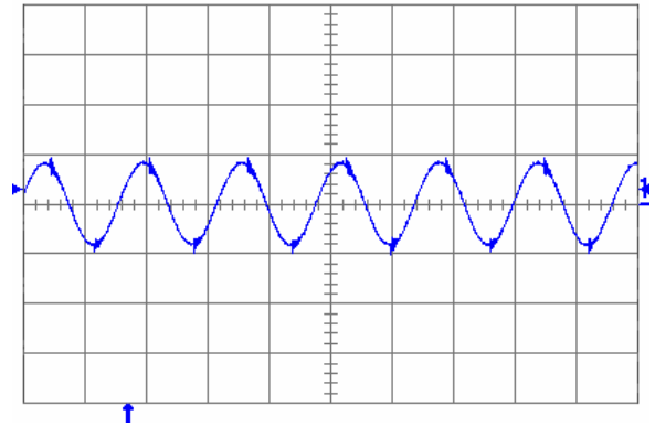
Fig. 2.0V.6: Output voltage ripple (20 mV/div.) at full rated load current into a resistive load with external capacitance 100\ \mu\text{F} ceramic + 1\ \mu\text{F} ceramic and V_{in} = 5\text{ V} for V_{out} = 2.0\text{ V} . Time scale: 2 \mu\text{s} /div.
