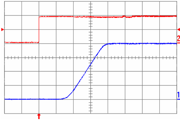
Fig. 2.0V.5: Turn-on transient for V_{out} = 2.0\text{ V} with the application of Enable signal at full rated load current (resistive) and 100\ \mu\text{F} external capacitance at V_{in} = 5\text{ V} . Top trace: Enable signal (2 V/div.); Bottom trace: output voltage (500 mV/div.); Time scale: 2 ms/div.
