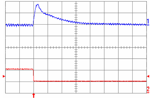
Fig. 1.2V.8: Output voltage response for V_{out} = 1.2\text{ V} to negative load current step change from 10\text{ A} to 5\text{ A} with slew rate of -5\text{ A}/\mu\text{s} at V_{in} = 5\text{ V} . Top trace: output voltage ( 100\text{ mV/div.} ); Bottom trace: load current ( 5\text{ A/div.} ). C_o = 100\text{ }\mu\text{F} ceramic + 1\text{ }\mu\text{F} ceramic. Time scale: 20\text{ }\mu\text{s/div.}
