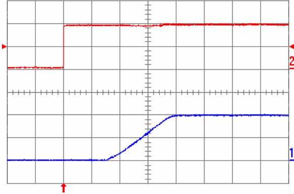
Fig. 1.0V.5: Turn-on transient for V_{out} = 1.0\text{ V} with the application of Enable signal at full rated load current (resistive) and 100\ \mu\text{F} external capacitance at V_{in} = 5\text{ V} . Top trace: Enable signal (2 V/div.); Bottom trace: output voltage (500 mV/div.); Time scale: 2 ms/div.
