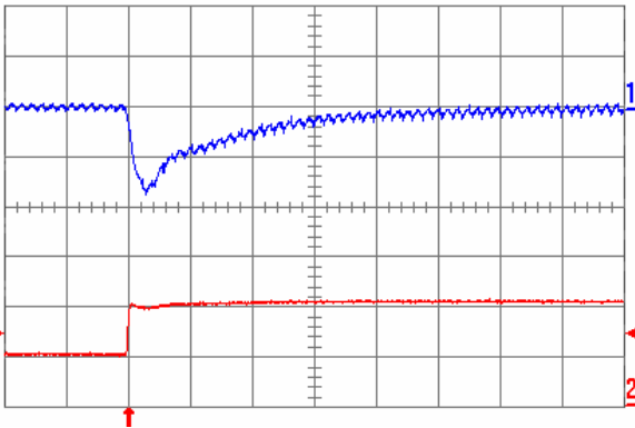
Fig. 1.2V.6: Output voltage response for V_{out} = 1.2\text{ V} to positive load current step change from 5\text{ A} to 10\text{ A} with slew rate of 5\text{ A}/\mu\text{s} at V_{in} = 5\text{ V} . Top trace: output voltage ( 100\text{ mV/div.} ); Bottom trace: load current ( 5\text{ A/div.} ). C_o = 100\text{ }\mu\text{F} ceramic + 1\text{ }\mu\text{F} ceramic. Time scale: 20\text{ }\mu\text{s/div.}
