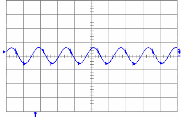
Fig. 1.2V.6: Output voltage ripple ( 20\text{ mV/div.} ) at full rated load current into a resistive load with external capacitance 100\text{ }\mu\text{F} ceramic + 1\text{ }\mu\text{F} ceramic and V_{in} = 5\text{ V} for V_{out} = 1.2\text{ V} . Time scale: 2\text{ }\mu\text{s/div.}
