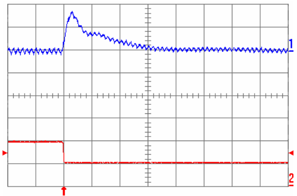
Fig. 1.8V.8: Output voltage response for V_{out} = 1.8\text{ V} to negative load current step change from 10 A to 5 A with slew rate of -5\text{ A}/\mu\text{s} at V_{in} = 5\text{ V} . Top trace: output voltage (100 mV/div.); Bottom trace: load current (5 A/div.). C_o = 100\ \mu\text{F} ceramic + 1\ \mu\text{F} ceramic. Time scale: 20 \mu\text{s} /div.
