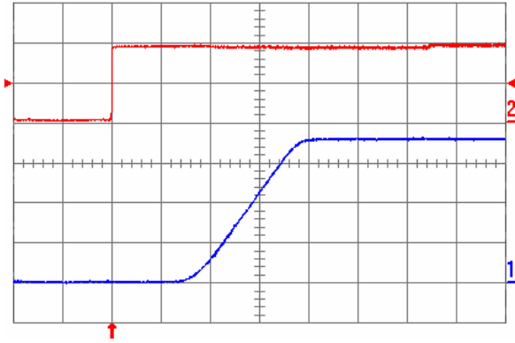
Fig. 1.8V.5: Turn-on transient for V_{out} = 1.8\text{ V} with the application of Enable signal at full rated load current (resistive) and 100\ \mu\text{F} external capacitance at V_{in} = 5\text{ V} . Top trace: Enable signal (2 V/div.); Bottom trace: output voltage (500 mV/div.); Time scale: 2 ms/div.
