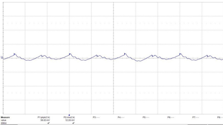
Fig. 49: Output voltage ripple (100 mV/div.) at full rated load current into a resistive load at V_{in} = 24V . Time: 2 \mu s /div.
