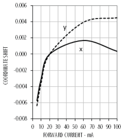
Figure 5 Chromaticity Shift vs. Forward Current
