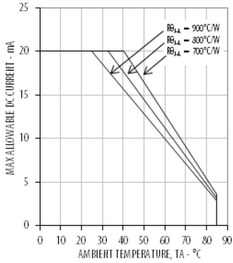
Figure 7 Derating Curve
