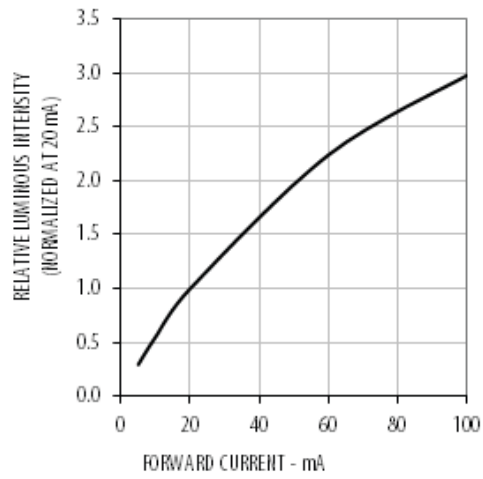
Figure 2 Relative Intensity vs. Forward Current
