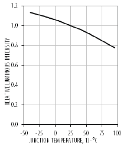
Figure 6 Relative Intensity vs. Temperature
