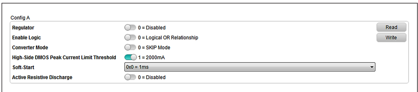
Figure 9. Config A Control Portion of Main GUI Window
