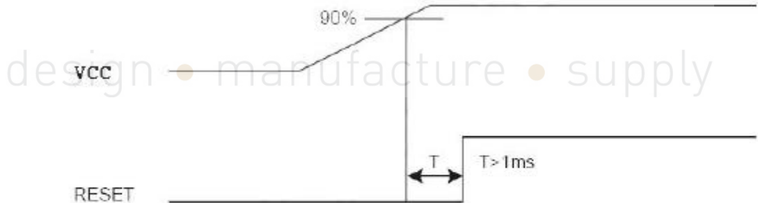
Reset timing
