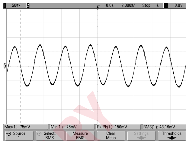
Figure 7. Ripple/Noise @+25°C (Vin=48V, Iout=50A, Cload=330µF, ScopeBW=20MHz, 2µS/div, 50mV/div)
