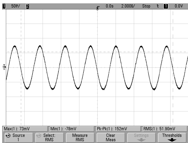
Figure 6. Ripple/Noise @+25°C (Vin=48V, Iout=0A, Cload=330µF, ScopeBW=20MHz, 2µS/div, 50mV/div)
