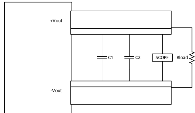
Figure 14. Measuring Output Ripple and Noise (PARD)
