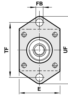
For Cylinder 9125
