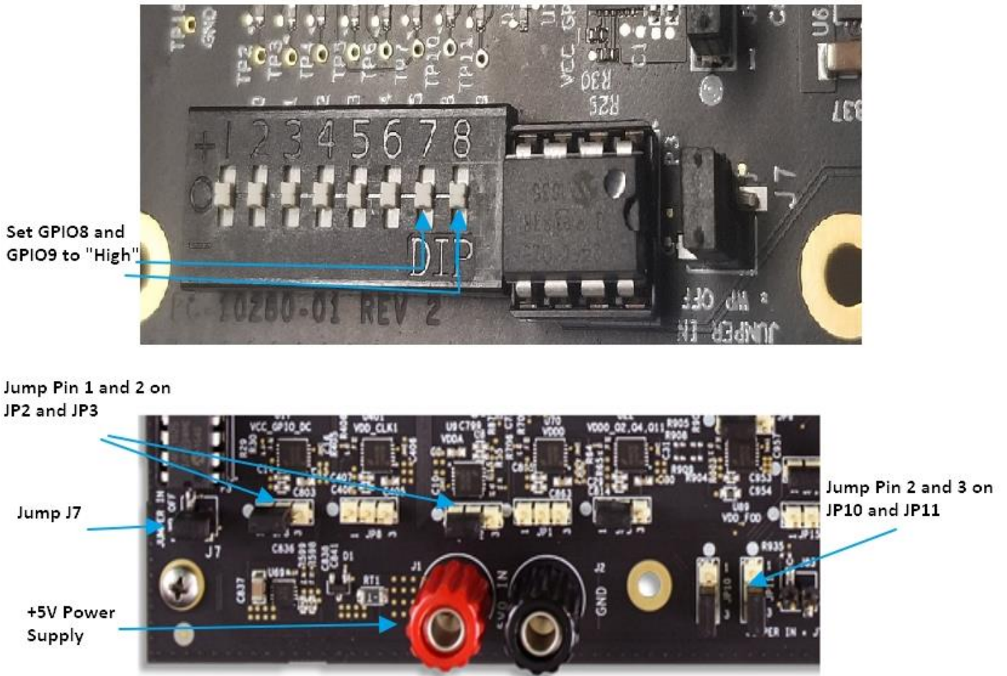
Figure 4. Board Setting for Default Operation
