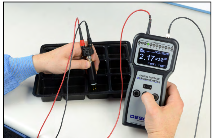
Figure 2. Using the Two-Point Resistance Probe with the Desco 19290 Digital Surface Resistance Meter
