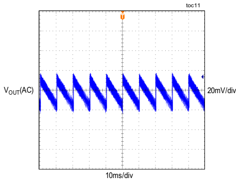
MAXM17624 OUTPUT VOLTAGE RIPPLE V_{IN} = 5V, V_{OUT} = 3.3V, I_{LOAD} = 1A, PFM \text{ MODE}
