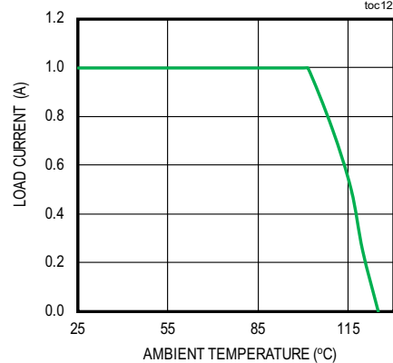
MAXM17624 OUTPUT CURRENT vs. AMBIENT TEMPERATURE V_{IN} = 5V, V_{OUT} = 3.3V, FULL \text{ LOAD}, PWM \text{ MODE}
