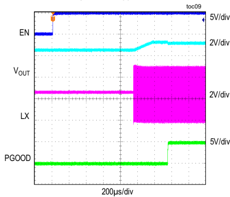
MAXM17624 STARTUP INTO PREBIAS V_{IN} = 5V, V_{PREBIAS} = 2.5V, V_{OUT} = 3.3V, PWM \text{ MODE}
