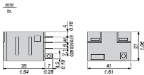
Pin Side View
