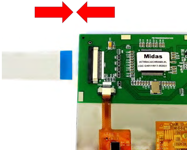
FIGURE 2 - CONNECT DISPLAY
