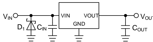
Figure 29. Surges Lower than -0.3 V is Applied to the Input
