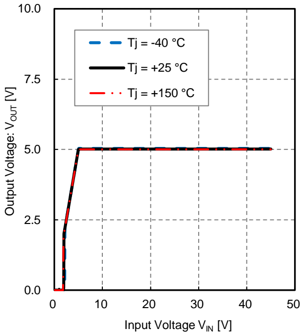
Figure 1. Output Voltage vs Input Voltage
