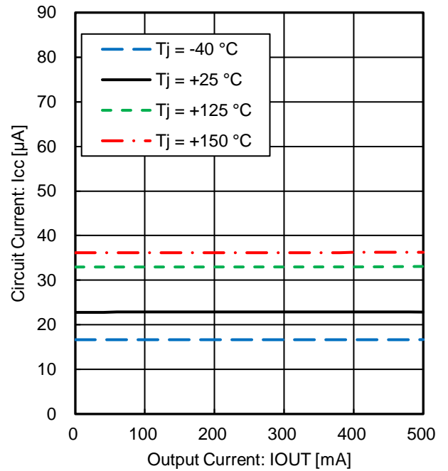
Figure 6. Current Consumption + Enable Bias Current vs Output Current
