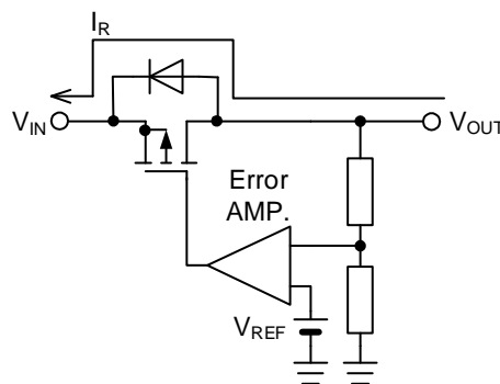
Figure 30. Reverse Current Path in a MOS Linear Regulator
