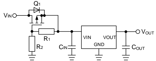
Figure 36. Protection against Reverse Polarity 3
