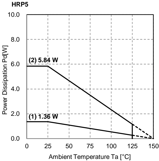
Figure 38. Power Dissipation Graph(HRP5)
