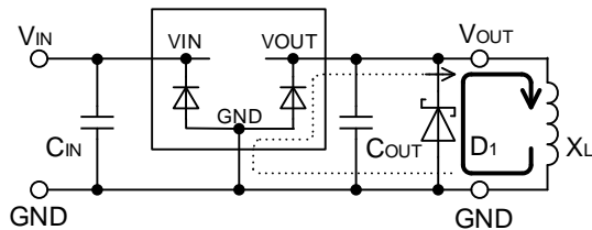
Figure 37. Current Path in Inductive Load (Output: Off)
