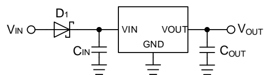
Figure 34. Protection against Reverse Polarity 1
