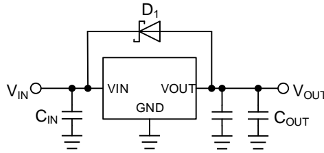
Figure 31. Bypass Diode for Reverse Current Diversion
