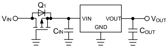
Figure 35. Protection against Reverse Polarity 2
