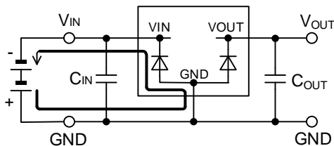
Figure 33. Current Path in Reverse Input Connection
