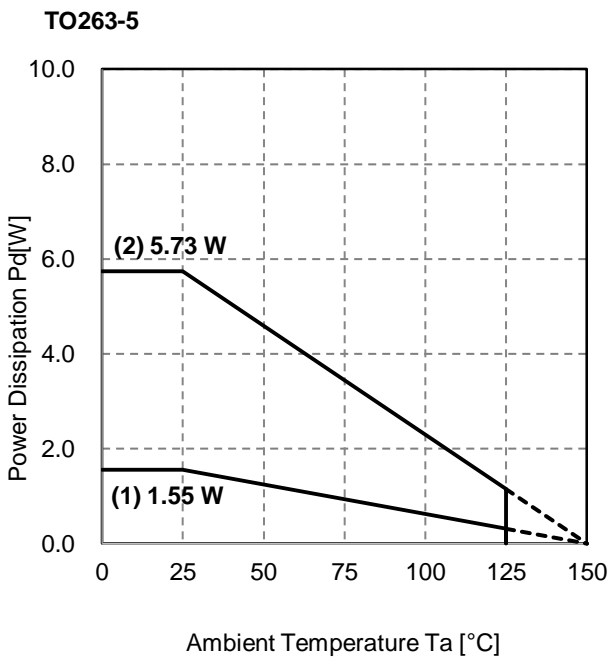
Figure 39. Power Dissipation Graph(TO263-5)
