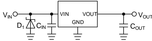
Figure 28. Surges Higher than absolute maximum ratings is Applied to the Input
