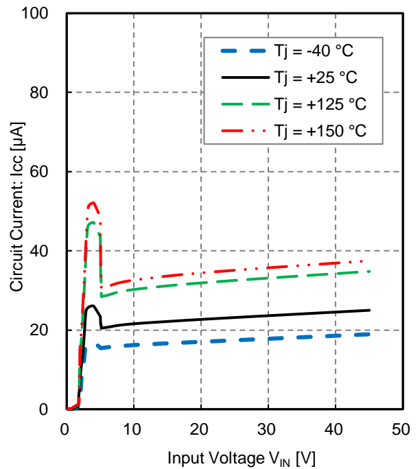
Figure 4. Current Consumption + Enable Bias Current vs Input Voltage
