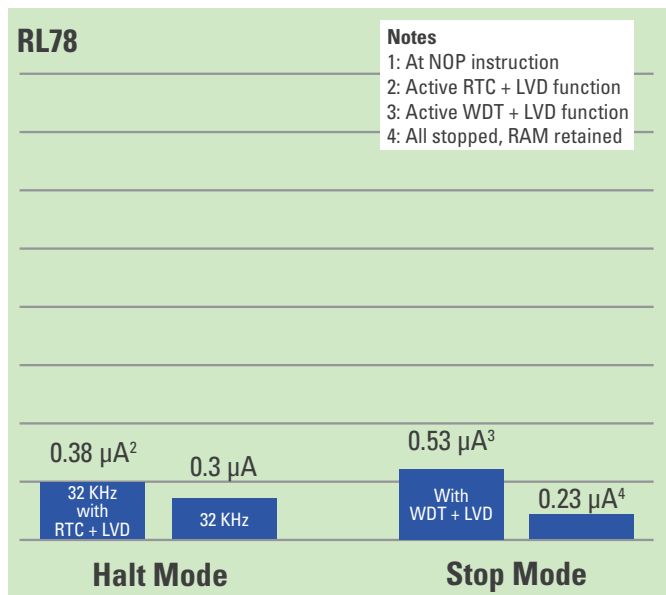
Figure 2 – RL78 Standby Current Consumption
