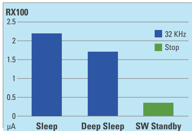
Figure 3 – RX100 Standby Current Consumption
