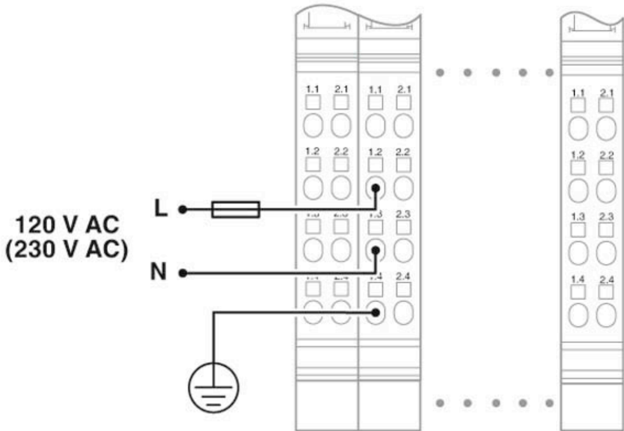
Connection diagram
