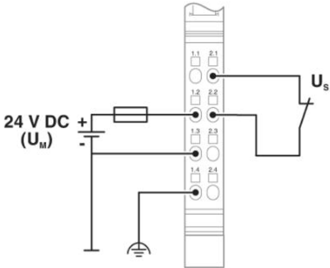
Connection diagram
