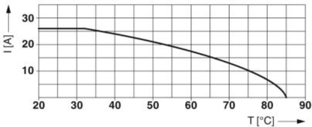
Nominal current depending on ambient temperature
