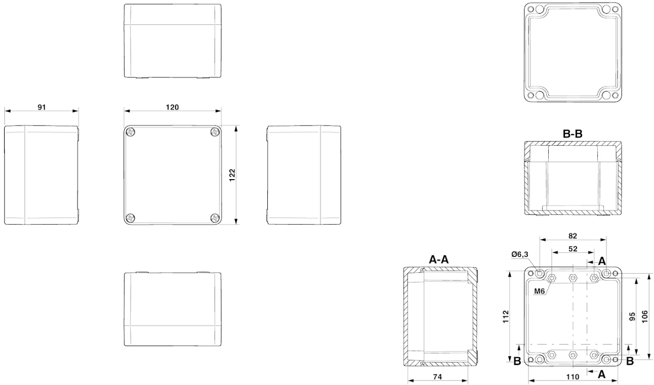
Dimensional drawing
