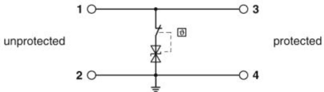
Circuit diagram
