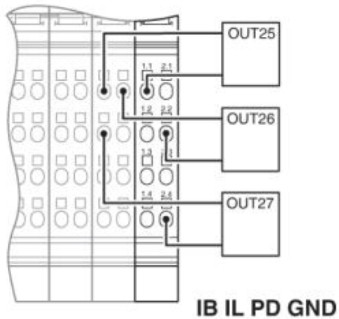
Connection diagram
