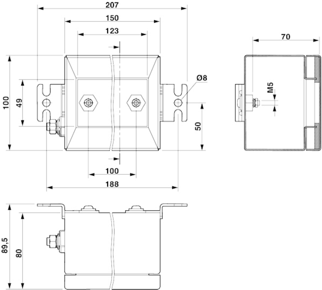
Dimensional drawing
