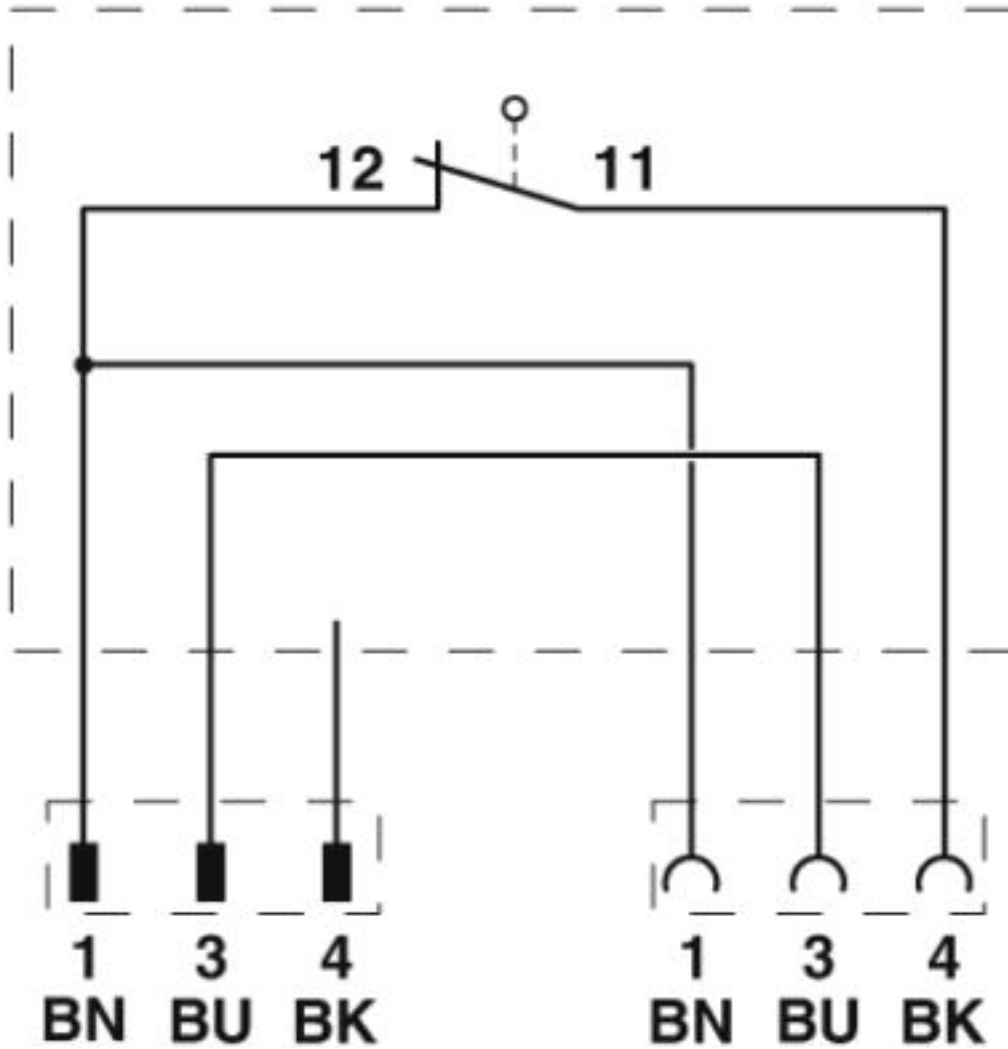
Circuit diagram
