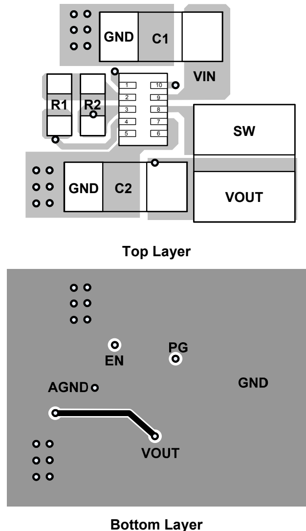
Figure 3: Layout Recommendation
