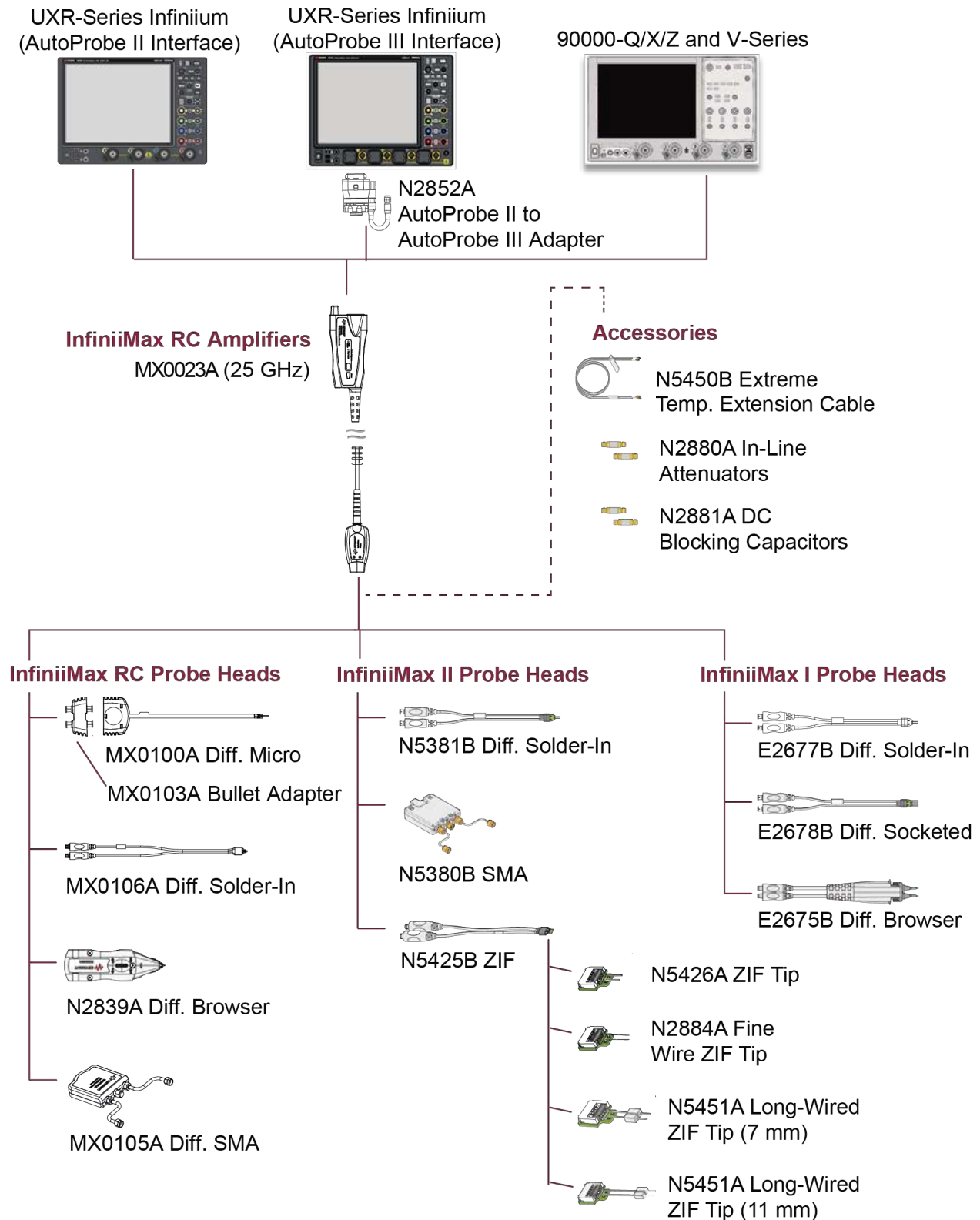
InfiniiMax RC probing system family diagram
