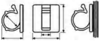
RB5-8 Self Adhesive Clip
