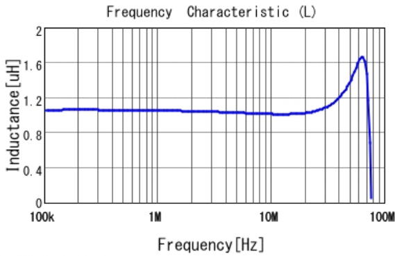
■ 1269AS-H-1R0M L
