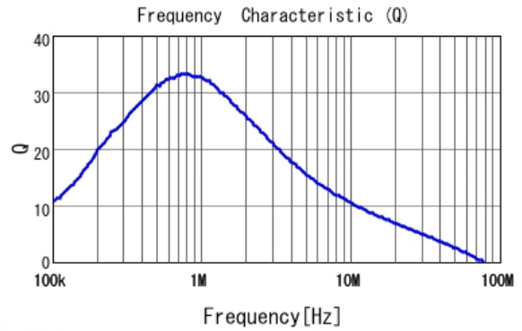
■ 1269AS-H-1R0M Q
