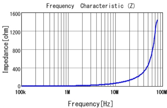
■ 1269AS-H-1R0M |Z|
