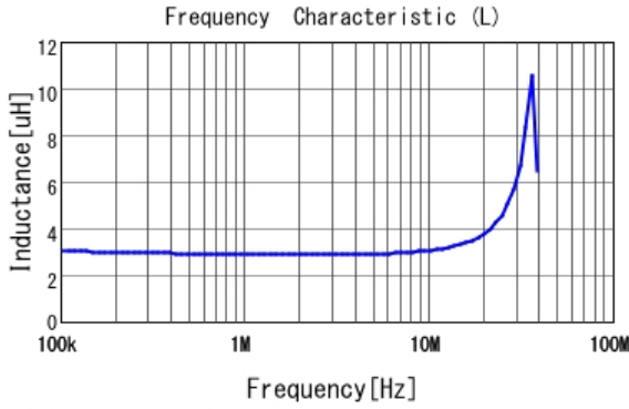
■ LQH5BPN3R3N38 L
