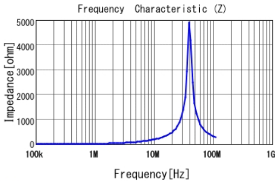
■ LQH5BPN3R3N38 |Z|
