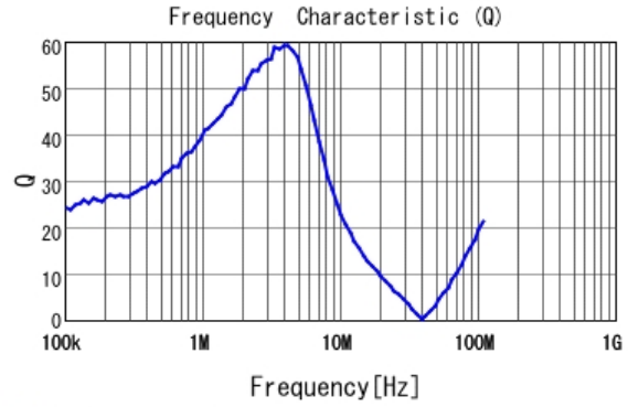
■ LQH5BPN3R3N38 Q
