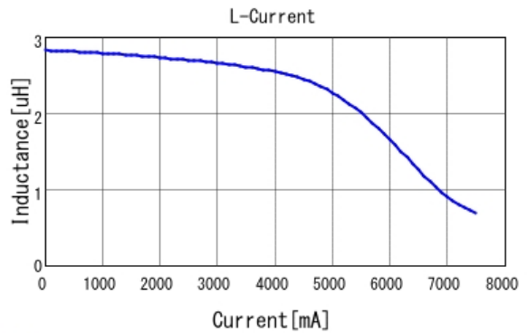
■ LQH5BPN3R3N38 L-Current 20degC
