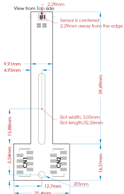
Figure 9: Mechanical Drawing LT Type 1 mil = 0.001in = 0.0254mm
